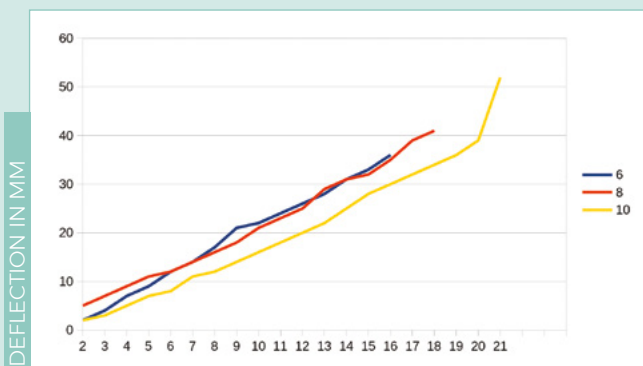
The deflection with force of bars with different numbers of perimeters
