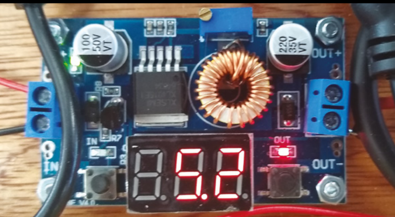
Below This switching regulator is powering our Raspberry Pi
