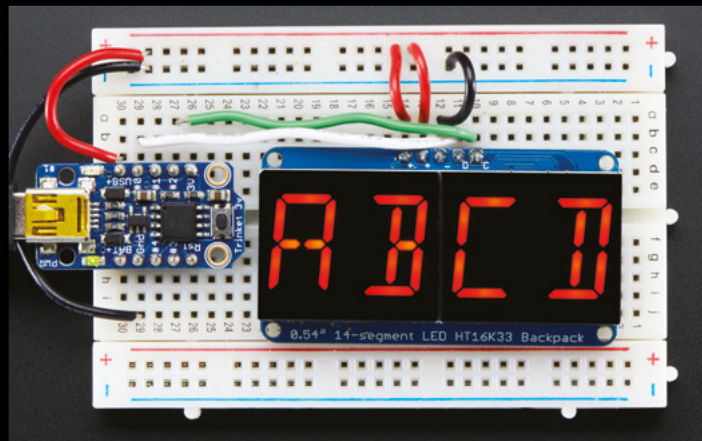
Below Here I 2 C is used to control an alphanumeric display using just two connections, data and clock
