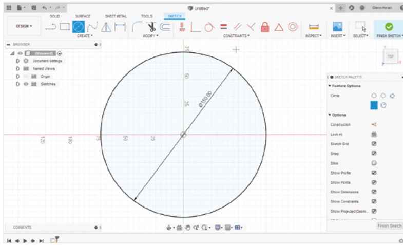
Figure 1 Once we've drawn our sketch, we get access to the sketch palette menu on the right to enter more parameters
