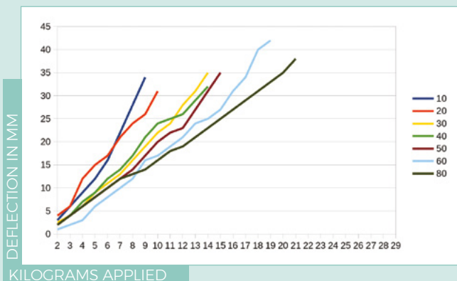
The deflection with force of bars with different amounts of infill
