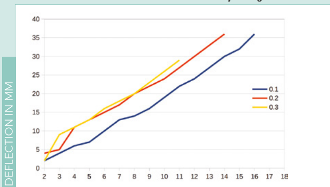
The deflection with force of bars with different layer heights
