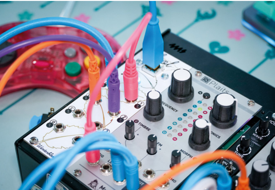
Above ■ Sol, Thea's first module, converts MIDI input into control voltage
