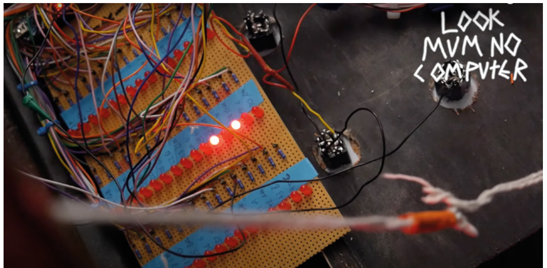
Below ♦ This perfboard circuit translates messages from the keyboard into trigger commands, telling the Furby to play a note
