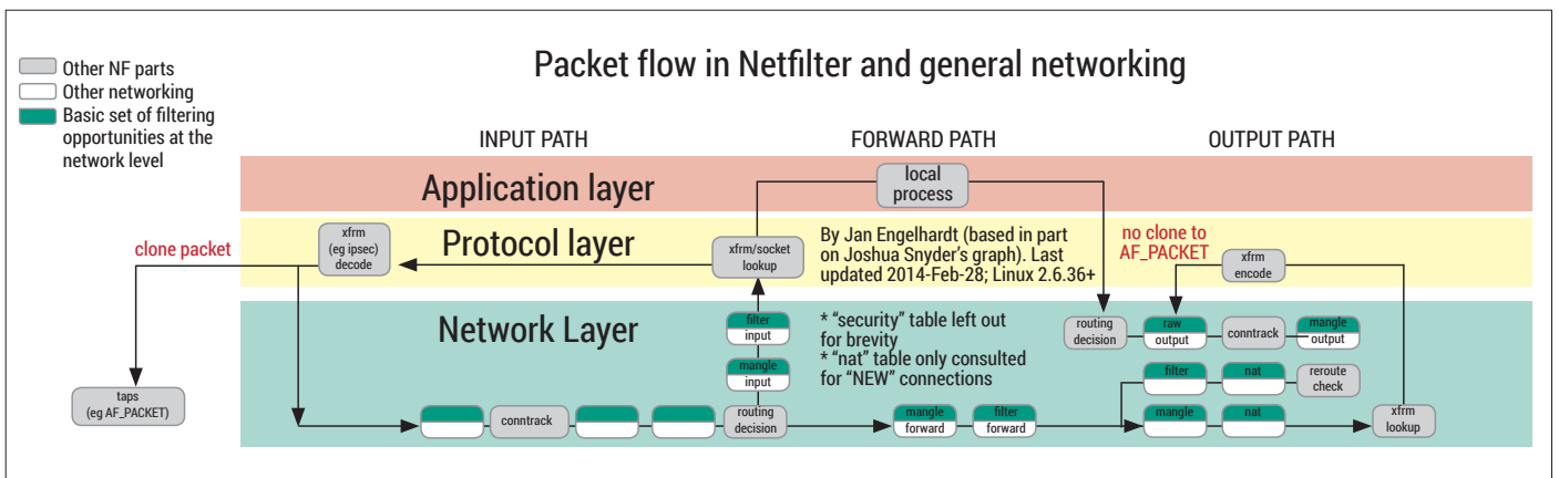
This diagram shows how network packets traverse built-in iptables chains and tables. Note that Netfilter is only part of the story.
