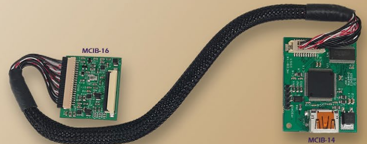
MCIB-16-LVDS-cable
