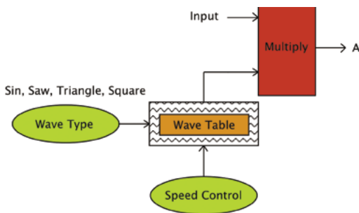
▼ Figure 7 Producing a Dalek effect
