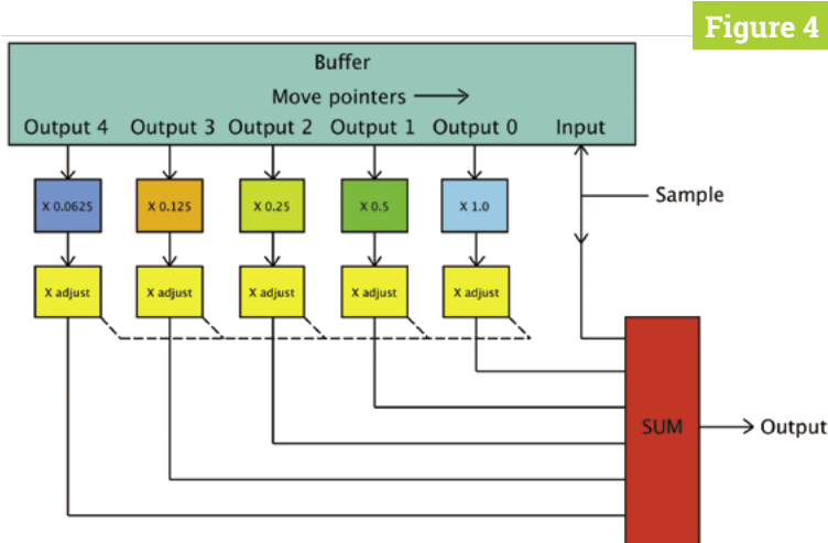
▲ Figure 4 Creating reverberation and echoes
