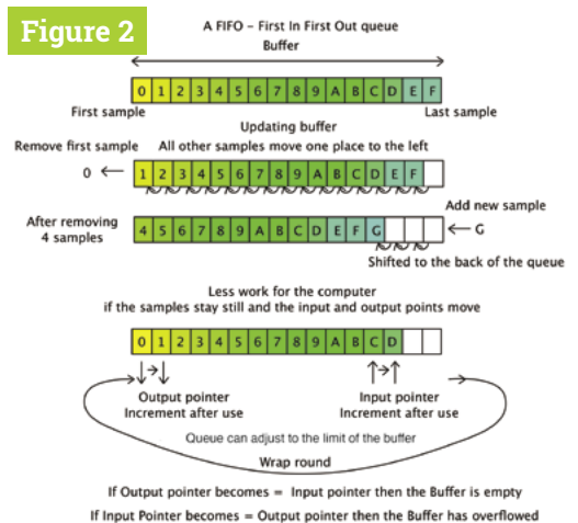
Figure 2 How a FIFO buffer works
