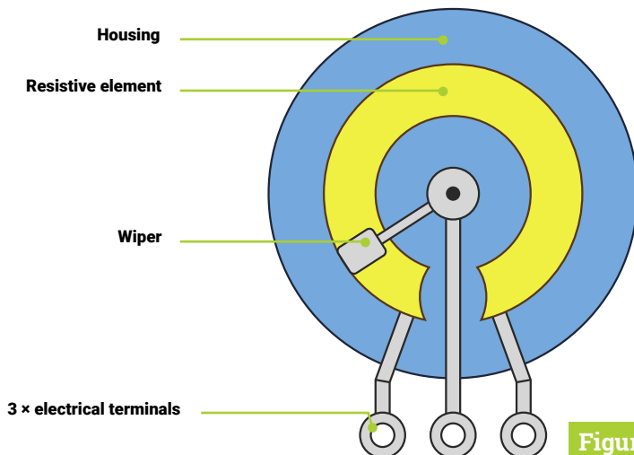
▼ Figure 2 How a potentiometer works
