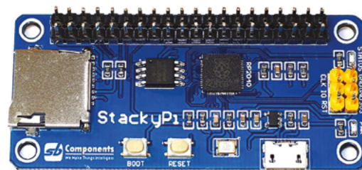
▲ The size of a Raspberry Pi Zero, the StackyPi is an RP2040-based microcontroller with a 40-pin GPIO header
