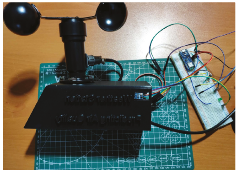
▲ Testing the weather station to make sure it all works
