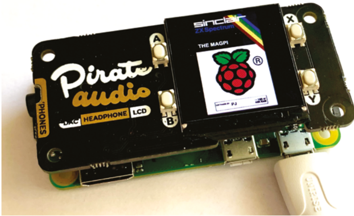
▲ The Pirate Audio HAT is a DAC (digital-to-analogue converter) combined with a small headphone amp
