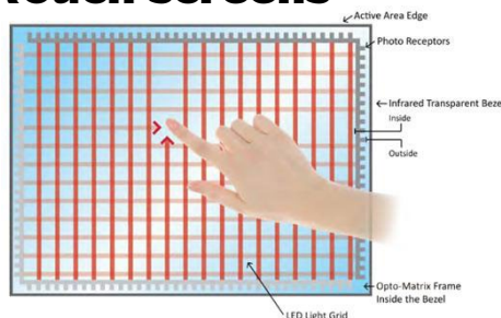
Principle of IR (Infrared) touch screen
