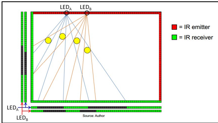
Principle of IR (Infrared) Multi-touch screen
