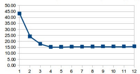
Linux kernel compilation with many threads[min]
