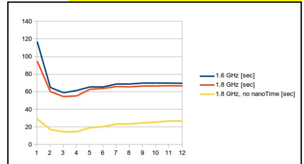
Over-clocking improves performance, but dropping usage of self-made instrumentation improves it significantly.
