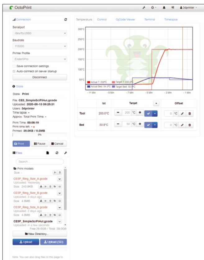
Figure 5: The web interface shows data for the printer – the temperature in this case. © Oliver Nickel
