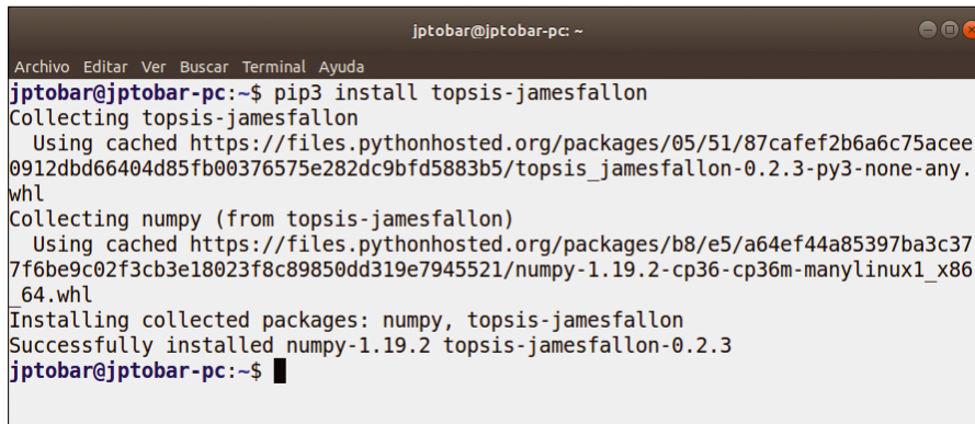
Figure 3: Installing topsis-python.
