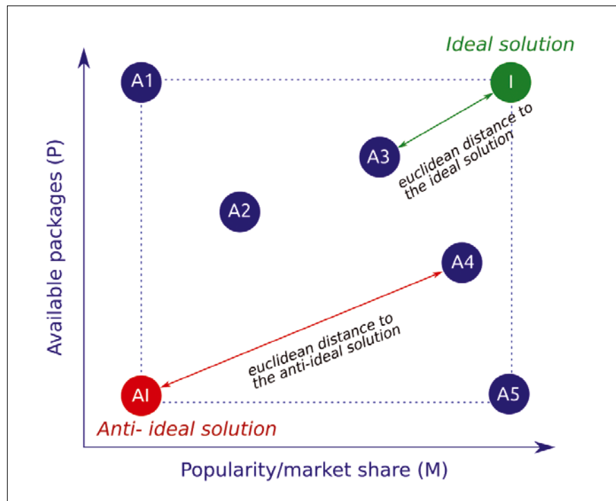
Figure 2: The TOPSIS technique.
