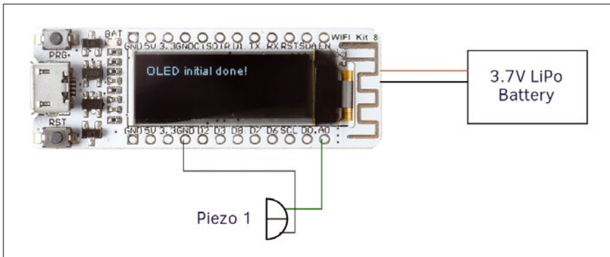
Figure 2: Schematic for the second version of the Nerf tower.
