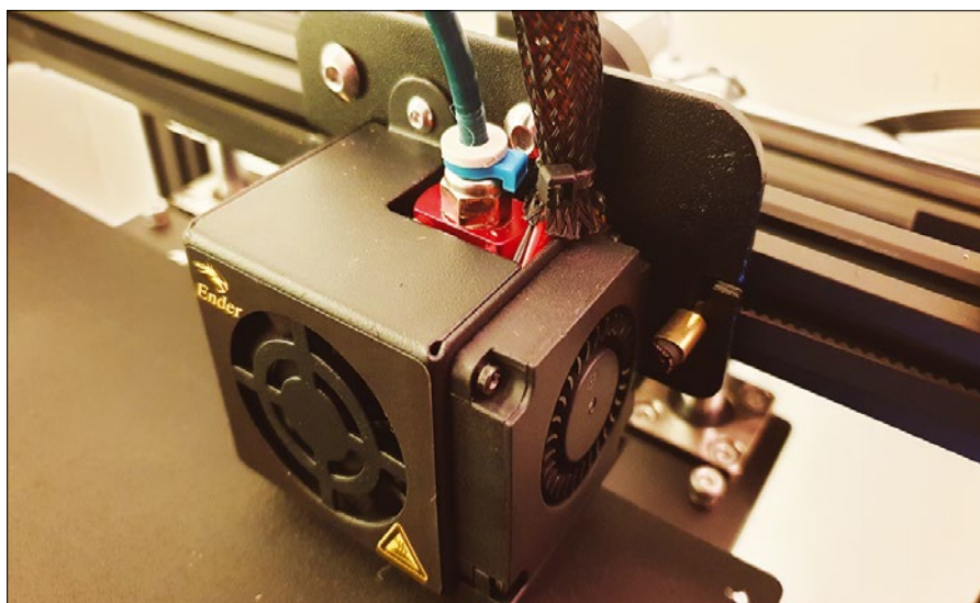
Figure 7: The Ender 5 Pro printhead was initially clogged. © Oliver Nickel
