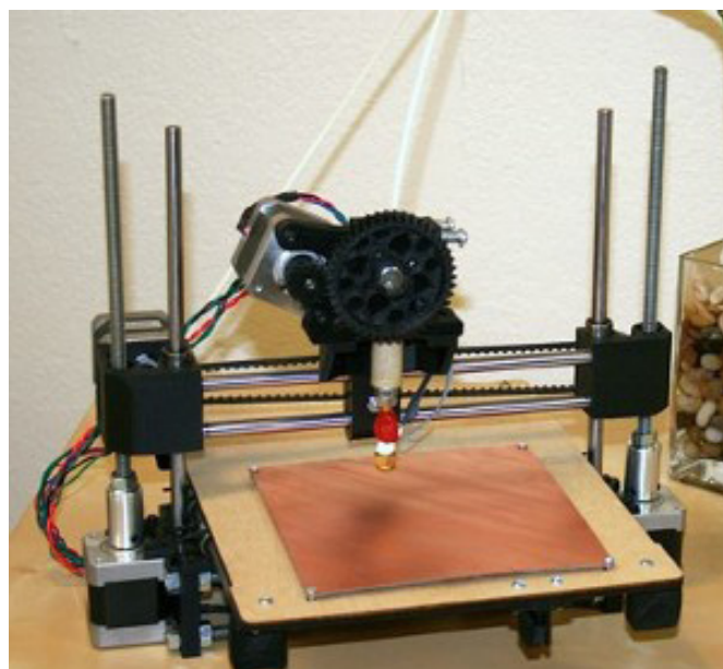
Printrbot (photo from http://printrbot.com )
