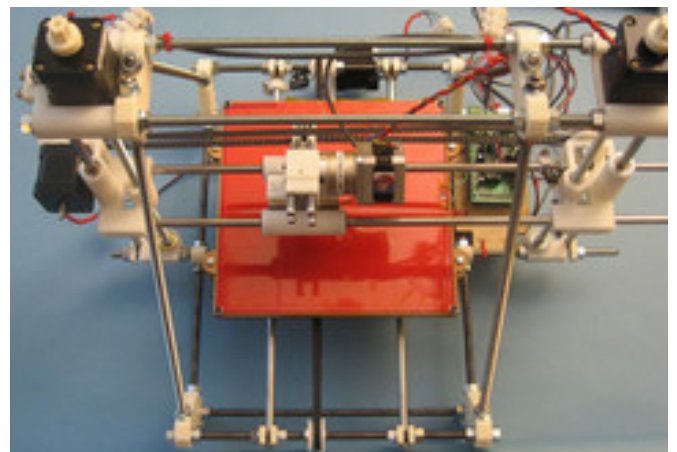
MakerGear (photo from http://www.makergear.com )
